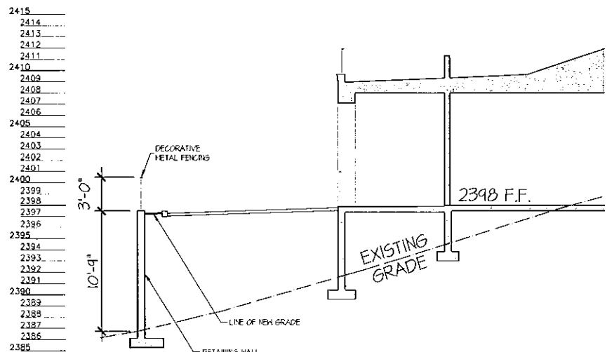
C RETAINING WALL SECTION SCALE: 3/16" = 1'-0"
