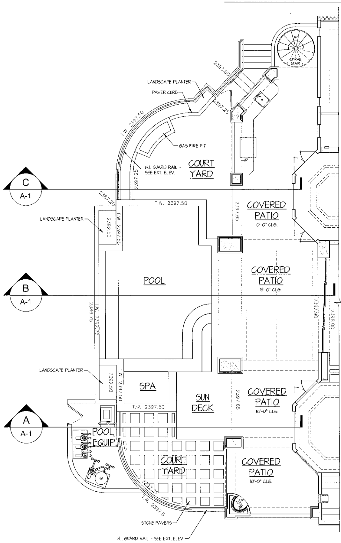
PARTIAL FLOOR PLAN SCALE: 1/4" = 1'-0"
