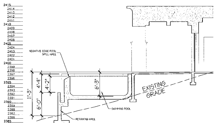
B RETAINING WALL SECTION SCALE: 3/16" = 1'-0"
