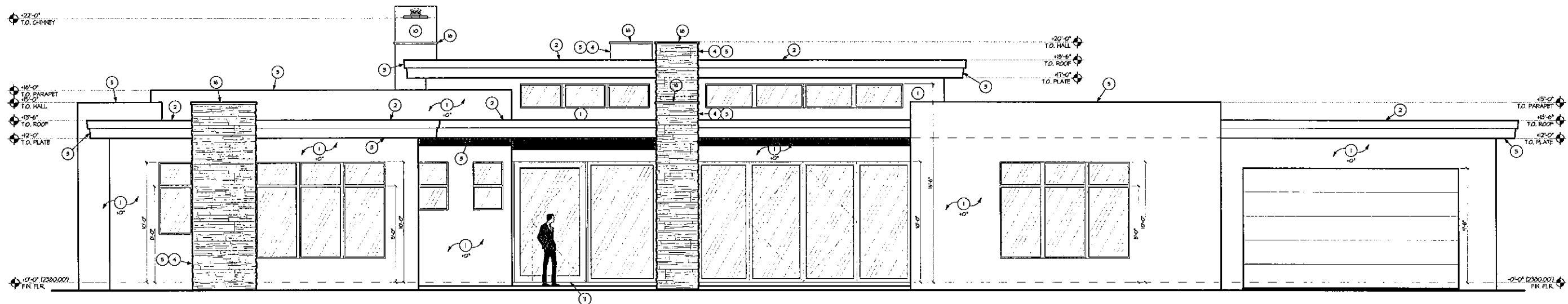
FRONT ELEVATION
