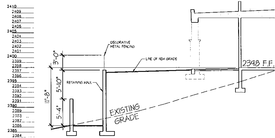
A RETAINING WALL SECTION SCALE: 3/16" = 1'-0"
