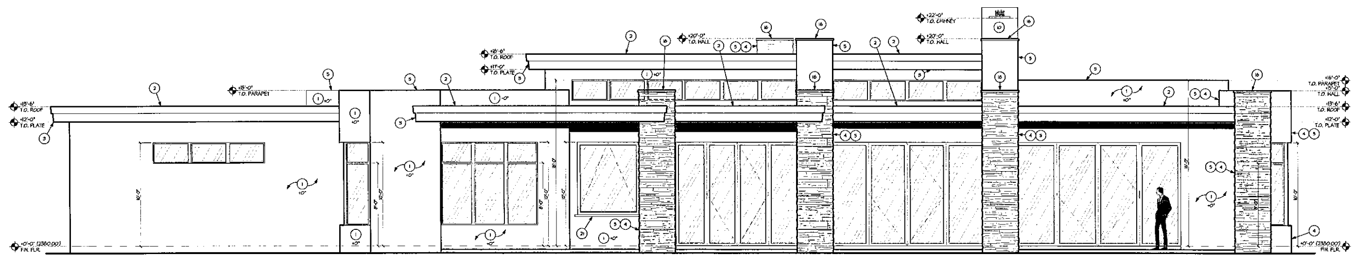
REAR ELEVATION
